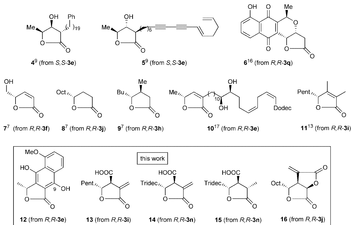
Scheme 2. \gamma -Lactone substitution patterns accessible from lactones of type 3: (–)-grandinoline (4), (–)-saproanthin (5), (+)-kalafungin (6), aglycon of (–)-ranunculin (7), (+)-dodecanolide (8), (–)-quercus lactone (9), (–)-montecristin (10), (+)-9-hydroxyeleutherol (12), (+)-methylenolactocin (13) and its enantiomer, (+)-protolichesterinic acid (14) and its enantiomer, (+)-rocellaric acid (15), and (–)-avenaciolide (16).
