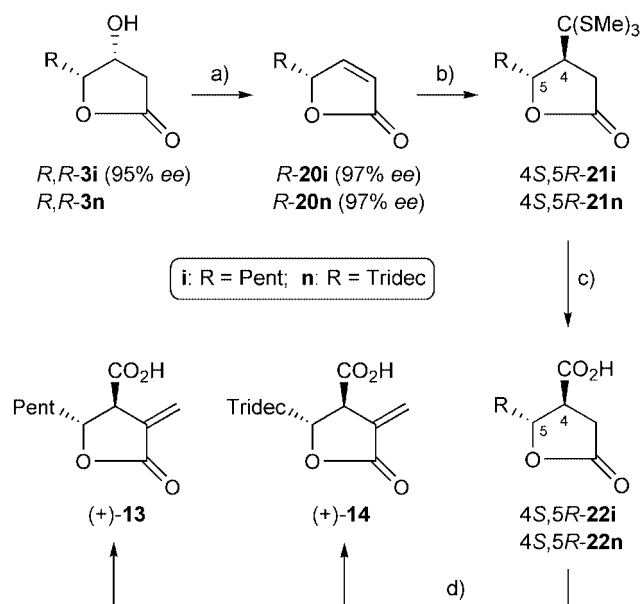
Scheme 4. Syntheses of (+)-methylenolactocin ( 13 ), (+)-protolichesterinic acid ( 14 ), and their (–) enantiomers (not depicted). Reagents and conditions: a) MsCl (1.1 equiv.), NEt 3 (2.1 equiv.), CH 2 Cl 2 , 0 °C, 15 min; 98% R-20i , 85% R-20n [enantiomeric series: analogously → 92% S - 20i , 83% S - 20n ]. b) HC(SMe) 3 (1.1 equiv.), THF, -78 °C, n BuLi (1.1 equiv.), 2–2.5 h; addition of R-20i or R-20n , respectively, 1.5–2 h; 90% (4 S ,5 R )- 21i , 85% (4 S ,5 R )- 21n [enantiomeric series: analogously → 93% (4 R ,5 S )- 21i , 86% (4 R ,5 S )- 21n ]. c) HgO (5.0 equiv.), THF/H 2 O (4:1), BF 3 ·OEt 2 (15 equiv.), room temp., 2.5 h; 93% (4 S ,5 R )- 22i , 91% (4 S ,5 R )- 22n [enantiomeric series: analogously → 94% (4 R ,5 S )- 22i , 93% (4 R ,5 S )- 22n ]. d) (i) MeOMg[O(C=O)OMe] (38 equiv.) in DMF, 135–140 °C, 70 h; isolation of the crude product; (ii) crude product from previous reaction, HOAc/NaOAc/formalin (= 35–40% aq. solution of formaldehyde)/ N -methylaniline (excess; 4:0.03:3:1), room temp., 2 h; 67% (+)- 13 , 72% (+)- 14 [enantiomeric series: analogously → 64% (–)- 13 (ref. [34] 66%), 68% (–)- 14 (ref. [30a] 68%)].
