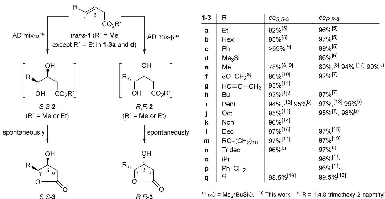
Scheme 1. Preparation of enantiopure \beta -hydroxy- \gamma -lactones by Sharpless' asymmetric dihydroxylation (AD) of \beta,\gamma -unsaturated carboxylic esters.
