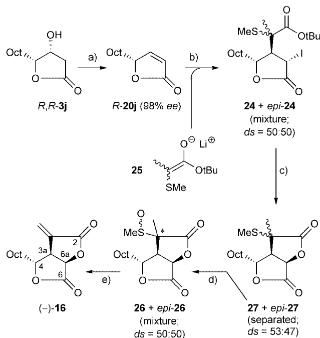
Scheme 6. Synthesis of (–)-avenaciolide ( 16 ). Reagents and conditions: a) MsCl (1.1 equiv.), NEt 3 (2.1 equiv.), CH 2 Cl 2 , 0 °C, 15 min; 83% (ref. [7] 91% and 95% ee ). b) 25 (1.1 equiv.), THF, –78 °C, addition of R - 20j , 3 h; I 2 (1.2 equiv.), 2 h; aq. HCl, –78 °C→0 °C; 82% (ref. [38] 93% for racemic material). c) p TsOH (0.4 equiv.), benzene, reflux, 3 h; aq. NaHCO 3 , room temp., 45 min; 47% 27 , 42% epi - 27 (ref. [38] 95% of a racemic mixture of these diastereomers). d) Starting from the pure diastereomer 27 : MCPBA (1.05 equiv.), CH 2 Cl 2 , 0 °C, 30 min; 81% of an inseparable mixture (50:50) of sulfoxide diastereomers. e) Mixture of sulfoxides from previous reaction, succinic anhydride (1.0 equiv.), 140 °C, 1 h; 75% (ref. [38] 73% starting from a racemic 26/epi-26 mixture).
