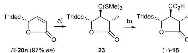
Scheme 5. Synthesis of (+)-rocellaric acid ( 15 ). Reagents and conditions: a) HC(SMe) 3 (1.1 equiv.), THF, -78 °C, n BuLi (1.1 equiv.), 1 h; addition of R-20n , 2 h; addition of MeI (3.0 equiv.), 4 h; → 92%. b) HgO (5.0 equiv.), BF 3 ·OEt 2 (15 equiv.), THF/H 2 O (4:1), room temp., 3 h; 93%.
