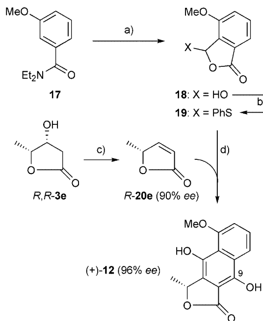
Scheme 3. Synthesis of (+)-9-hydroxyeleutherol ( 12 ). Reagents and conditions: a) 17 and TMEDA (1.1 equiv.) in Et 2 O, -78 °C; addition of s BuLi (1.1 equiv.) over 1 h, -78 °C, 1 h; addition of DMF (1.2 equiv.), 1 h, room temp.; aq. KOH (2 M), 12 h; 51% (ref. [26] 66%). b) PhSH (1.2 equiv.), p TsOH (cat.), benzene, reflux, azeotropic removal of water, 6 h; 79% (ref. [26] 85%). c) MsCl (1.1 equiv.), NEt 3 (2.1 equiv.), CH 2 Cl 2 , 0 °C, 20 min; 89% (ref. [8] 70%, 94% ee). d) THF/DMSO (1:1), 0 °C, addition of MeLi (1.1 equiv.); addition of 19 in DMSO, 30 min; addition of R-20e , 5 h; 56%.
